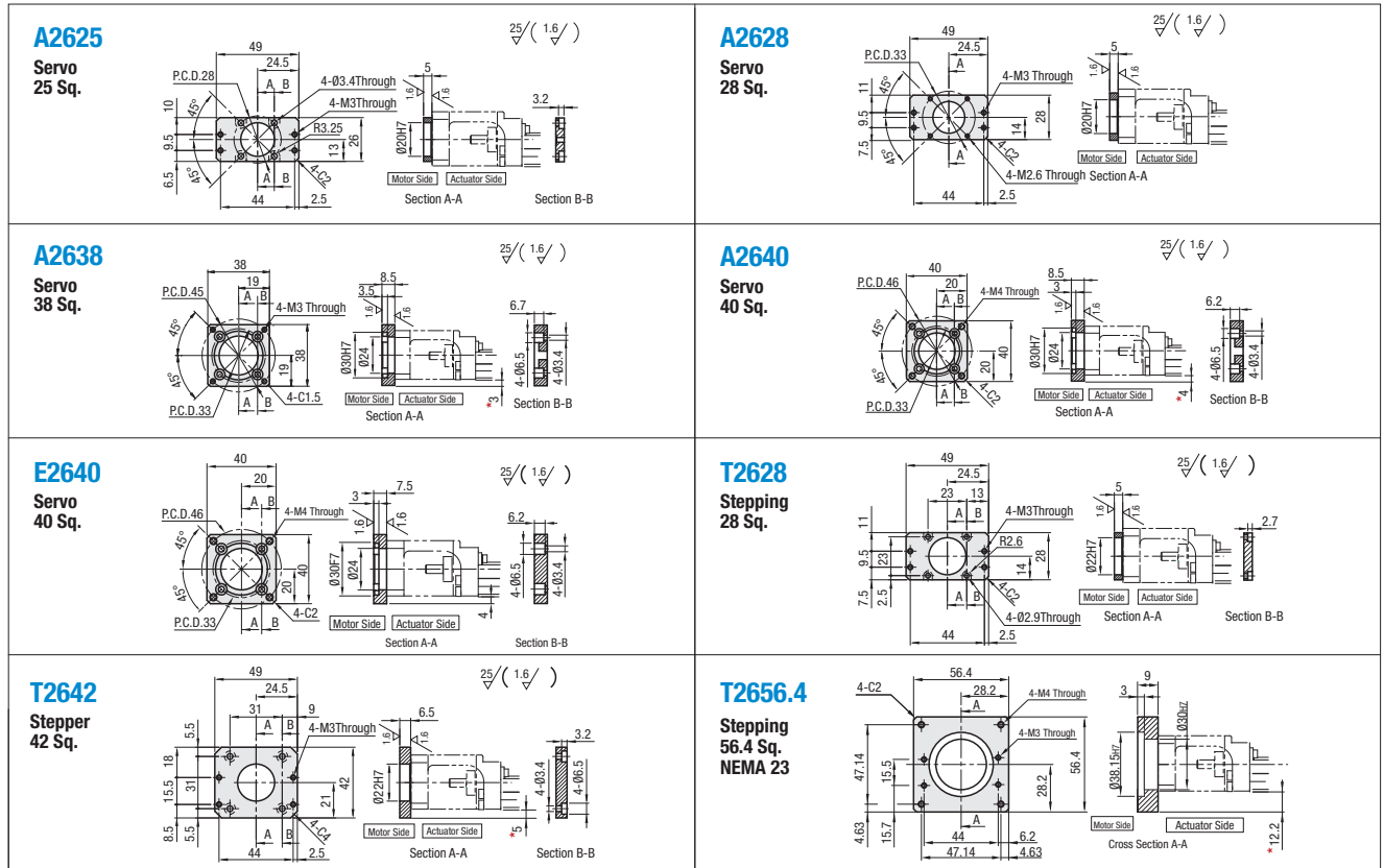
Servo Motor Application Table
